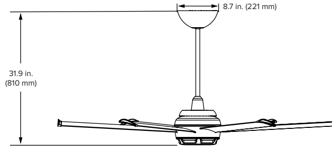
Shown with the 20 in. (508 mm) downrod. See the full fan cut sheet for a complete list of fan heights with optional downrods.
